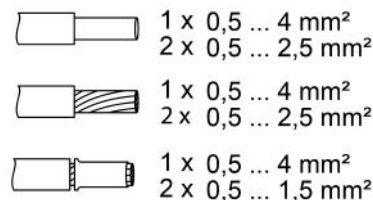
Figure 4: Clampable conductor cross-section
